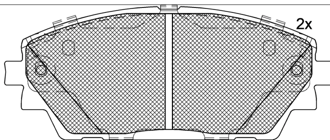
Loose Shim
